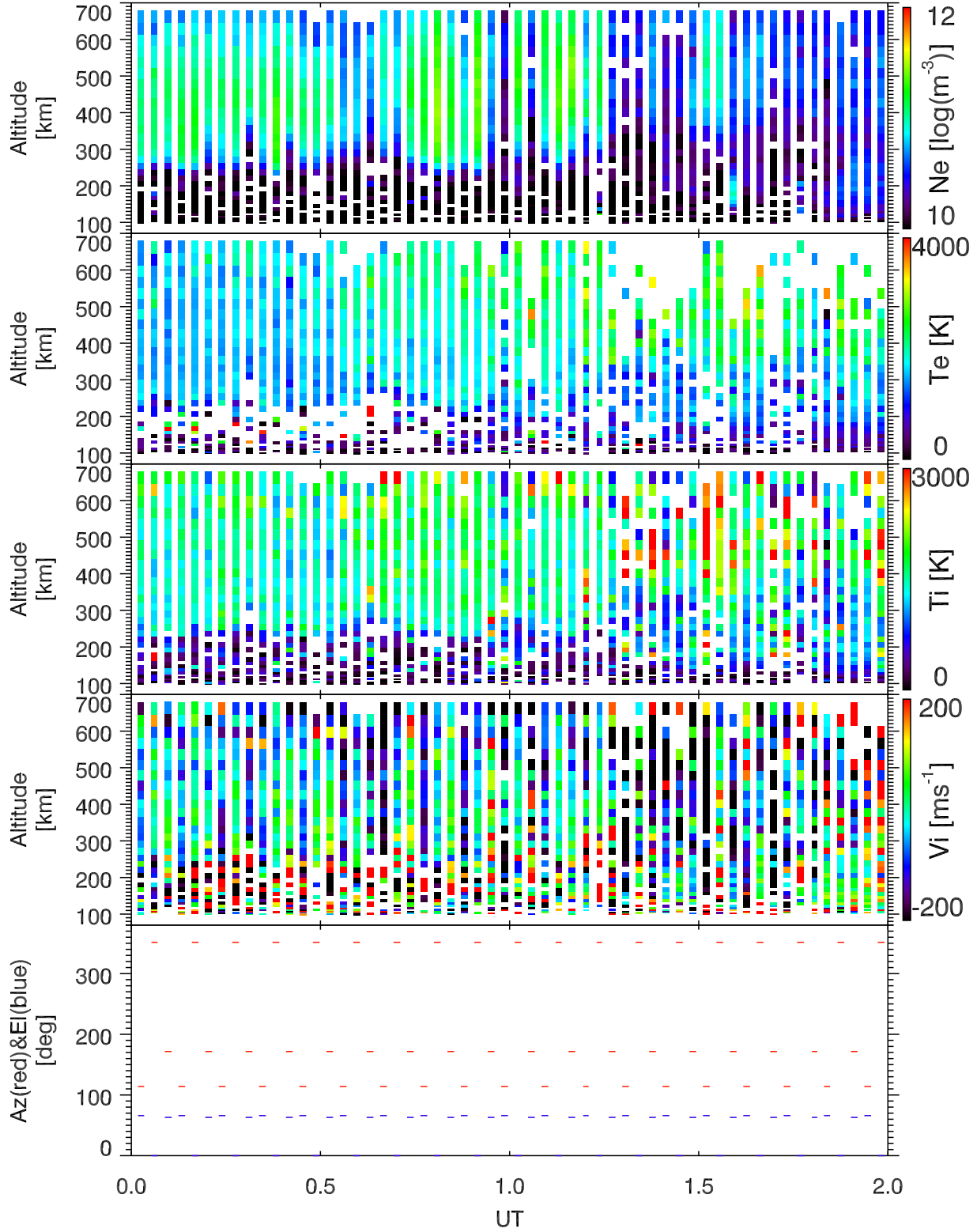
EISCAT 2002-10-12_00_02UT_tau0_ant@32m.
