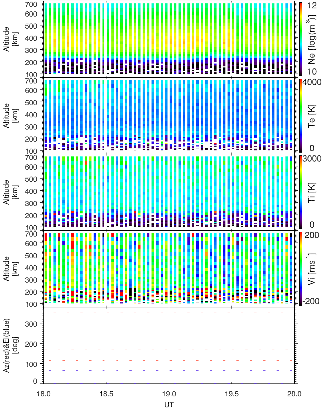
EISCAT 2002-10-12_18_20UT_tau0_ant@32m.
