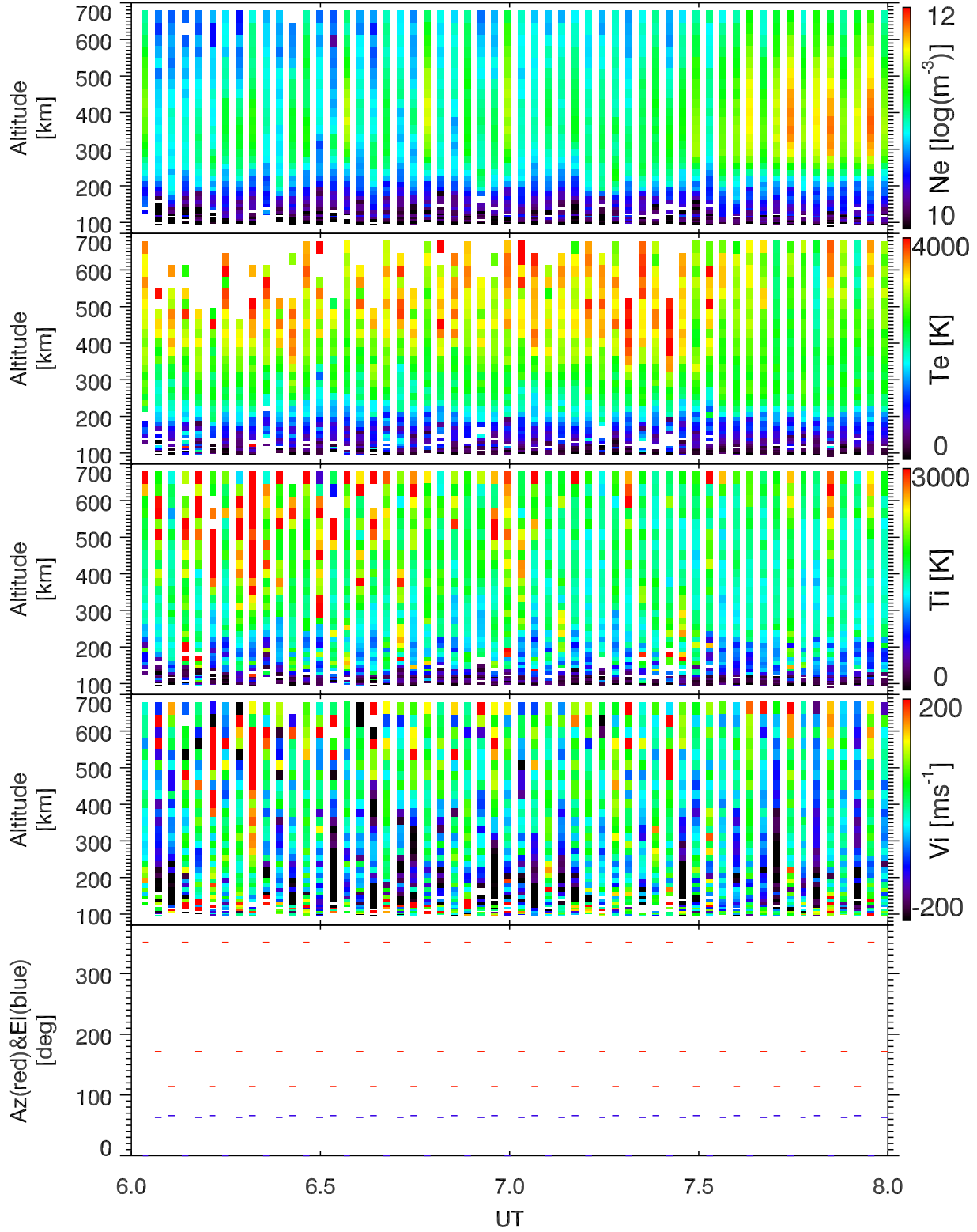
EISCAT 2002-10-13_06_08UT_tau0_ant@32m.
