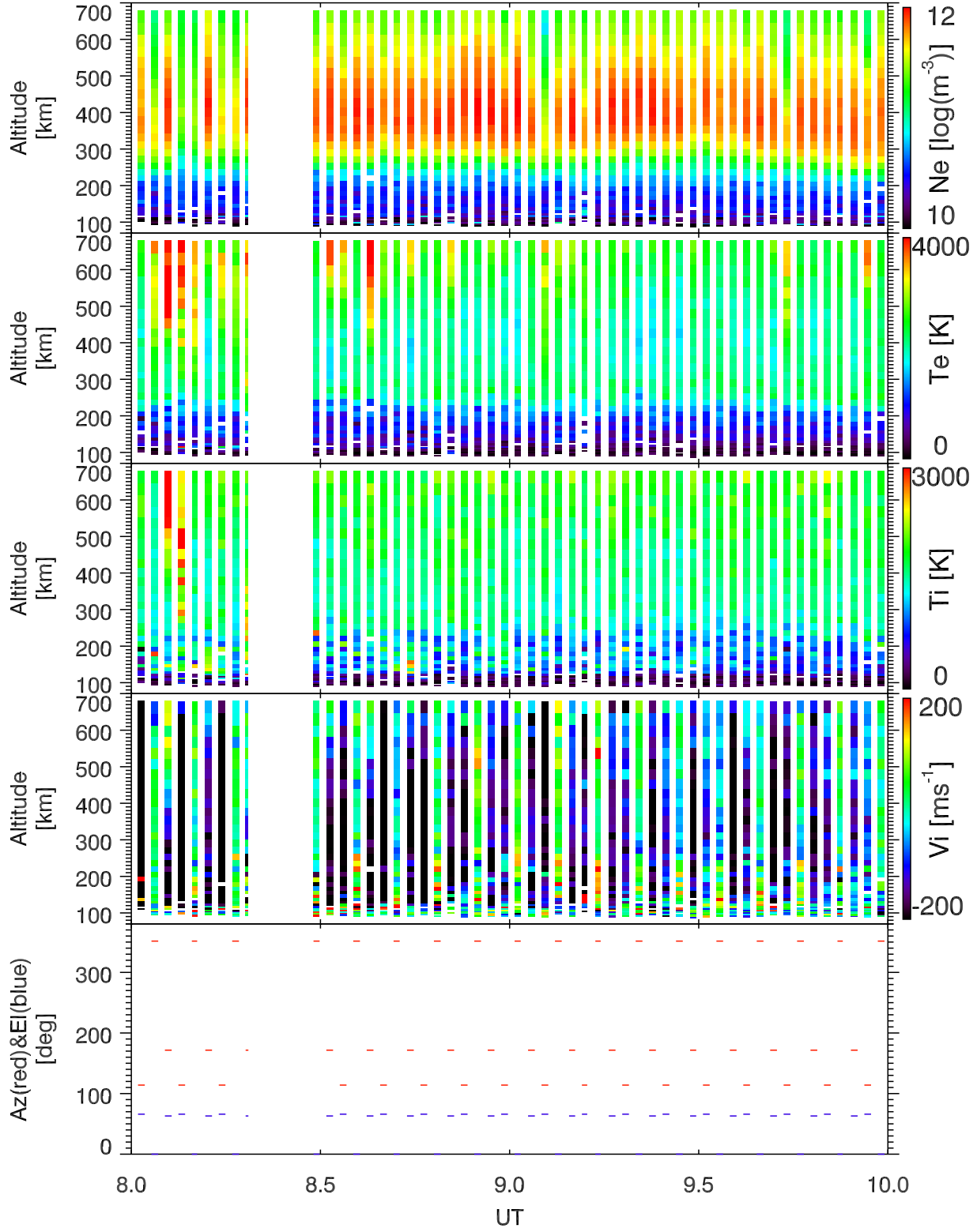
EISCAT 2002-10-14_08_10UT_tau0_ant@32m.
