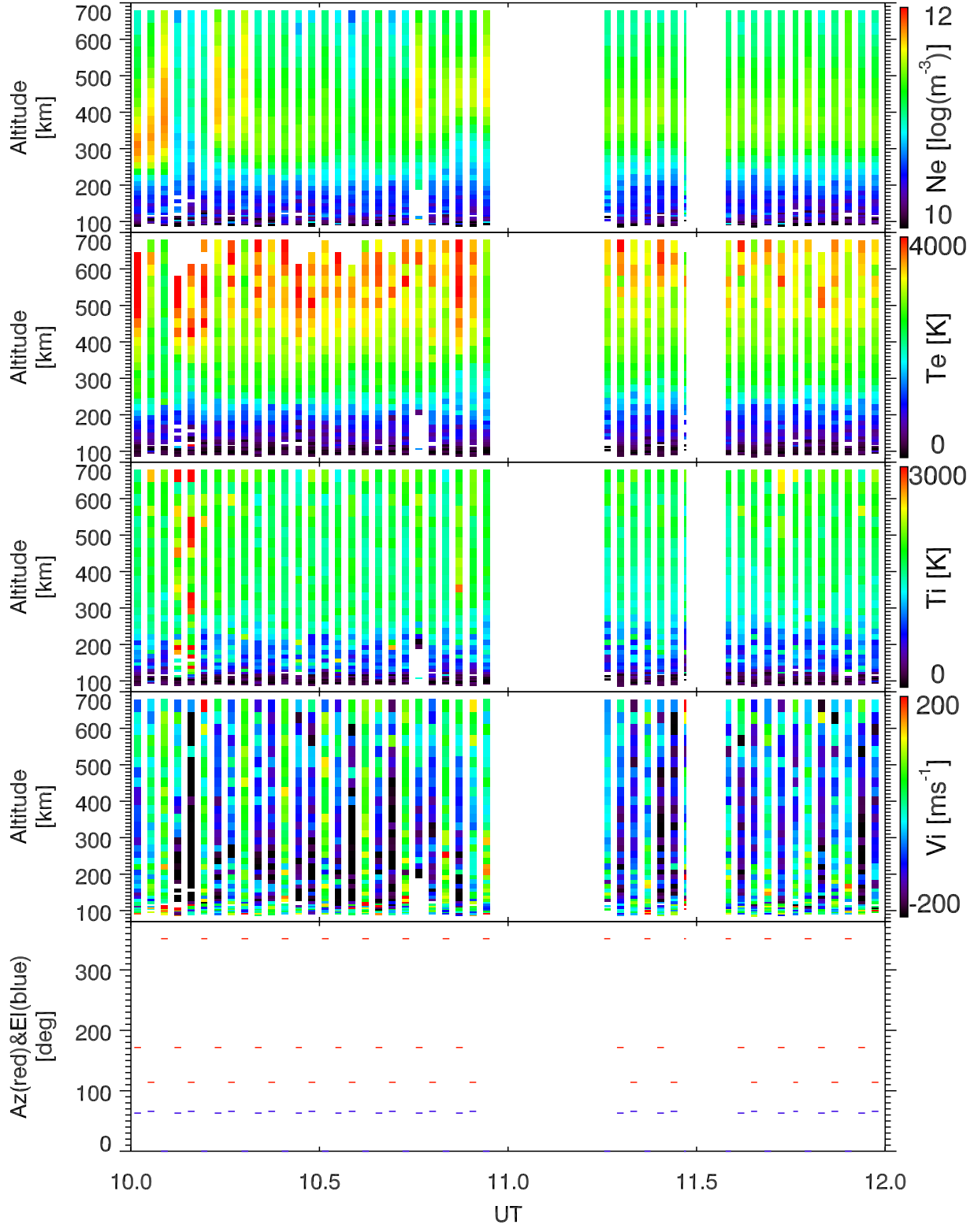
EISCAT 2002-10-14_10_12UT_tau0_ant@32m.
