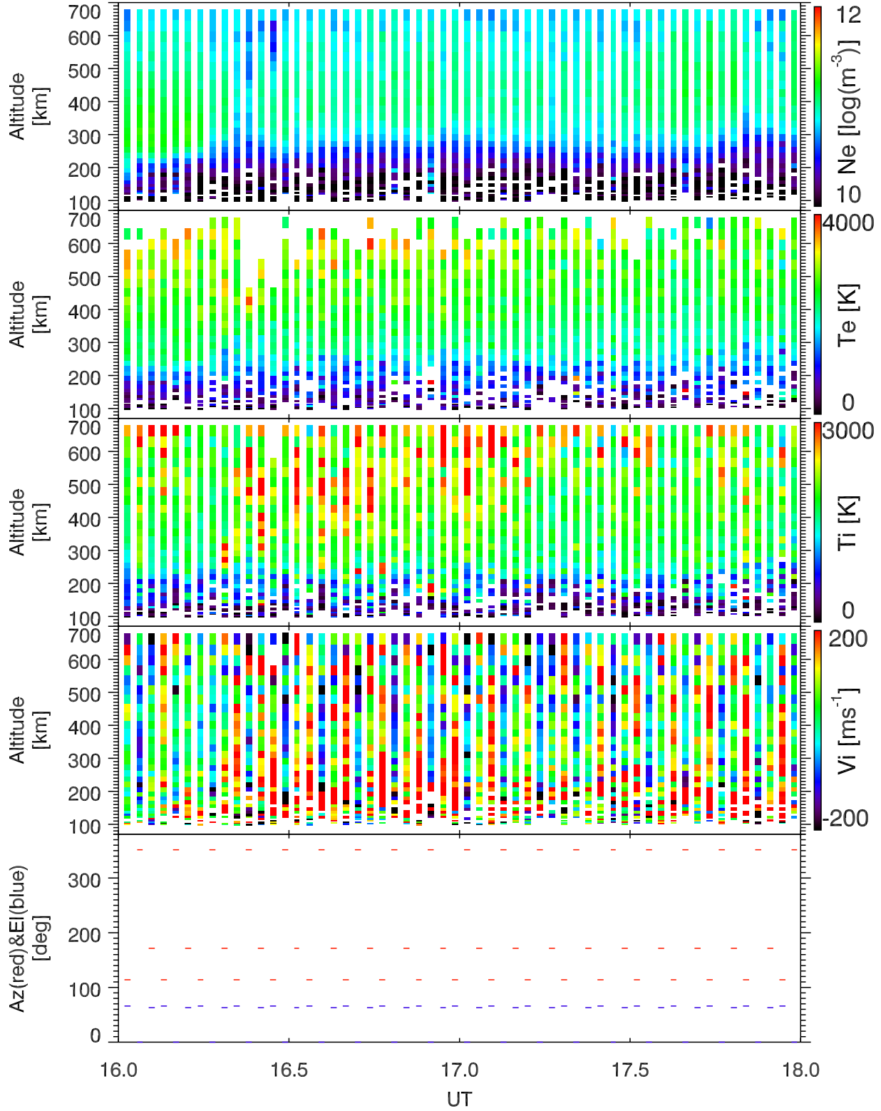
EISCAT 2002-10-14_16_18UT_tau0_ant@32m.
