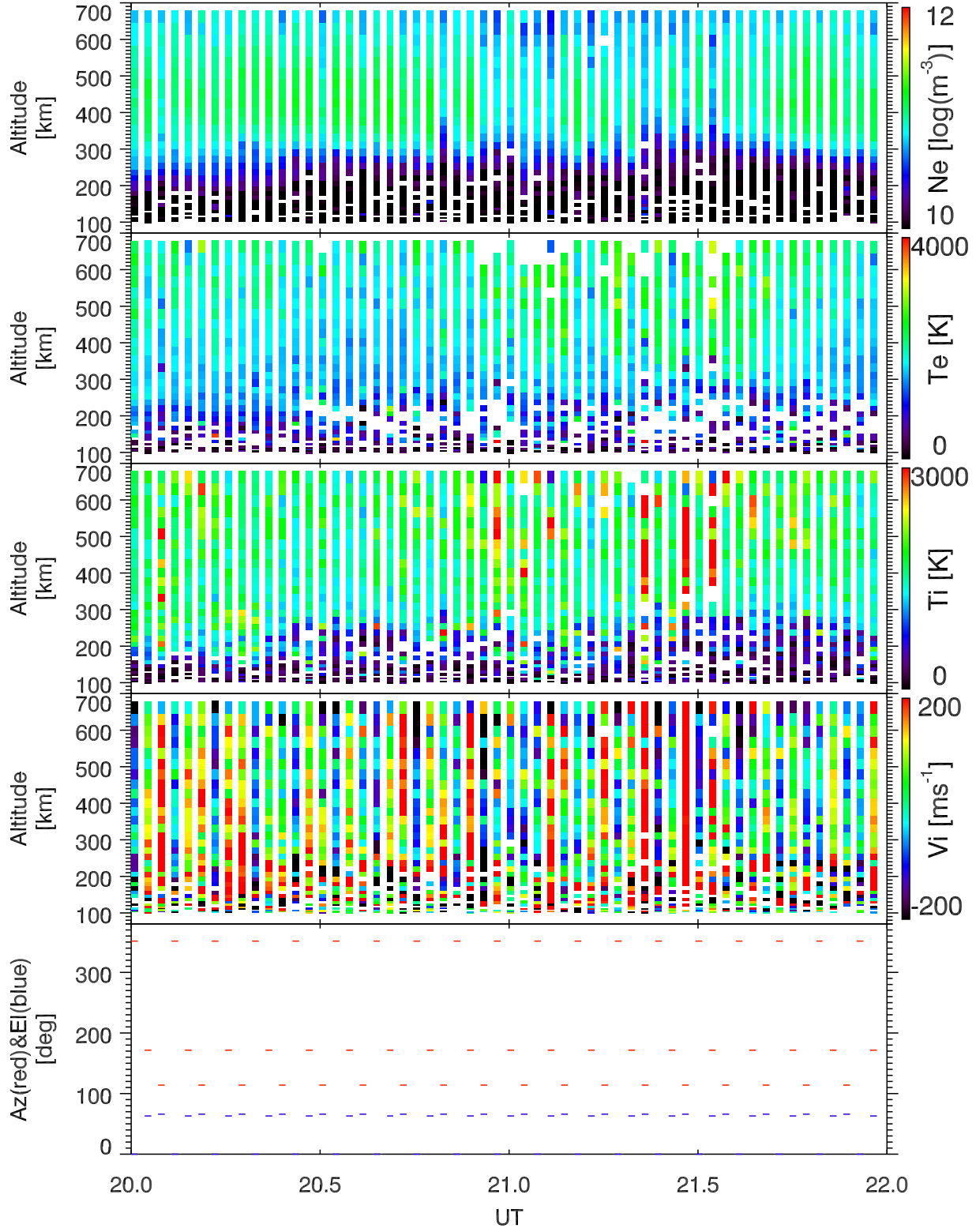
EISCAT 2002-10-14_20_22UT_tau0_ant@32m.
