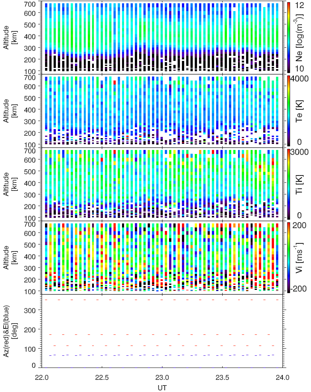
EISCAT 2002-10-14_22_24UT_tau0_ant@32m.
