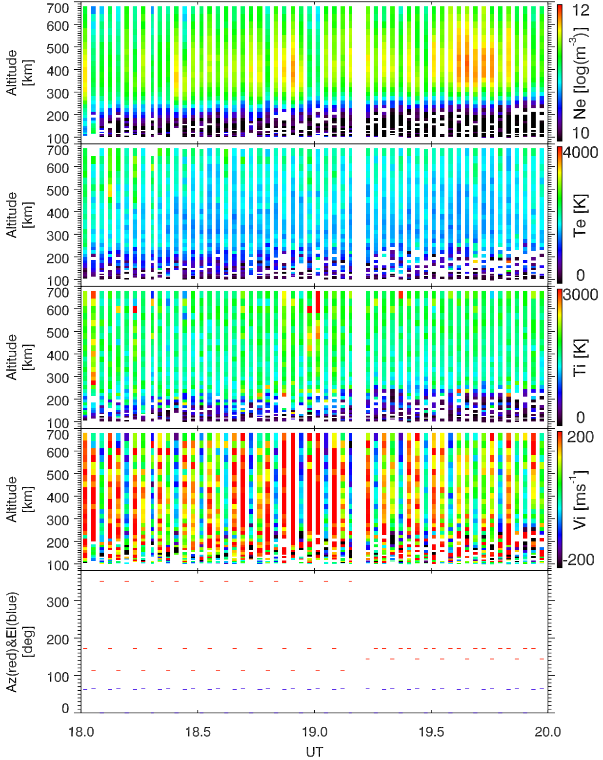
EISCAT 2002-10-15_18_20UT_tau0_ant@32m.
