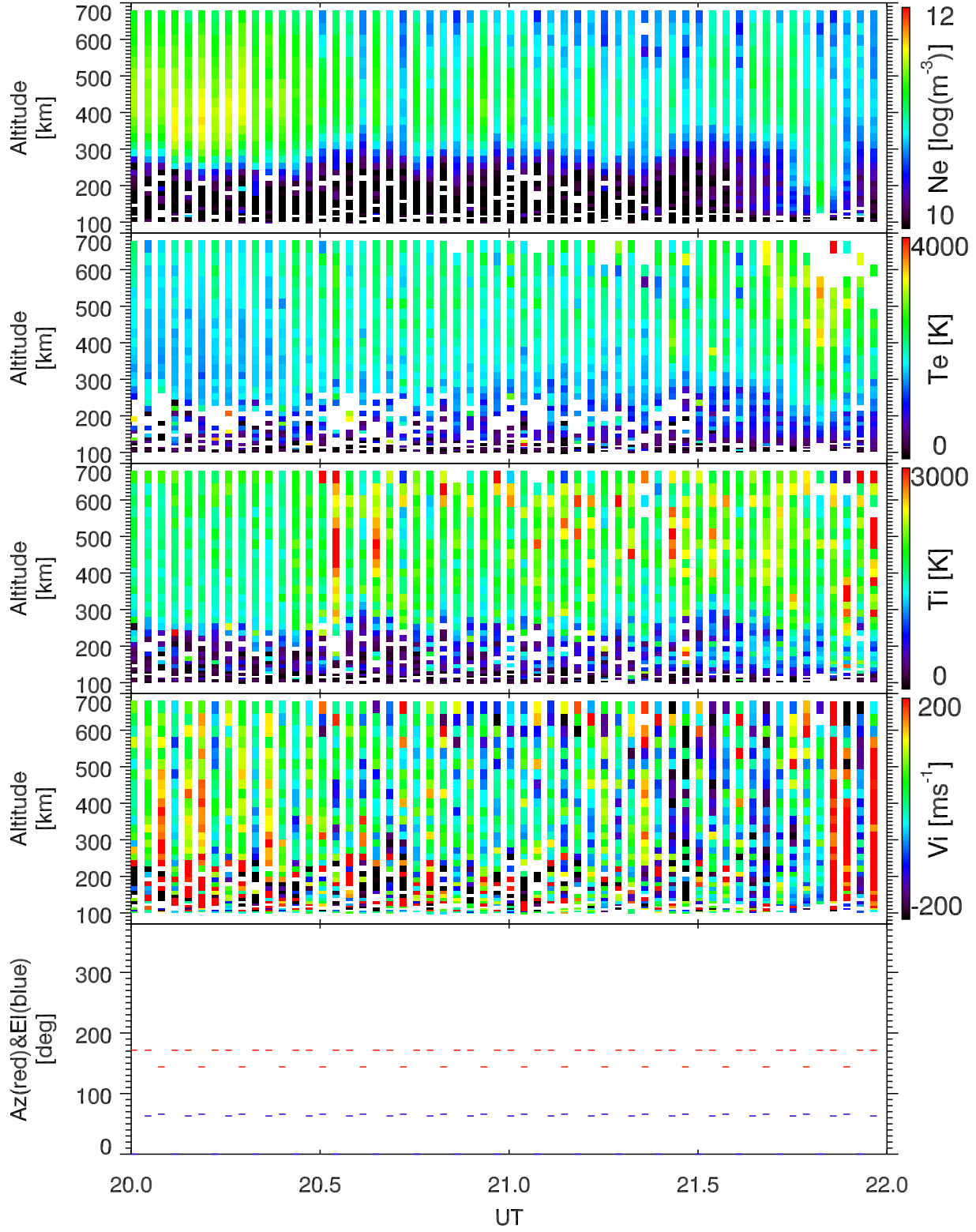
EISCAT 2002-10-15_20_22UT_tau0_ant@32m.
