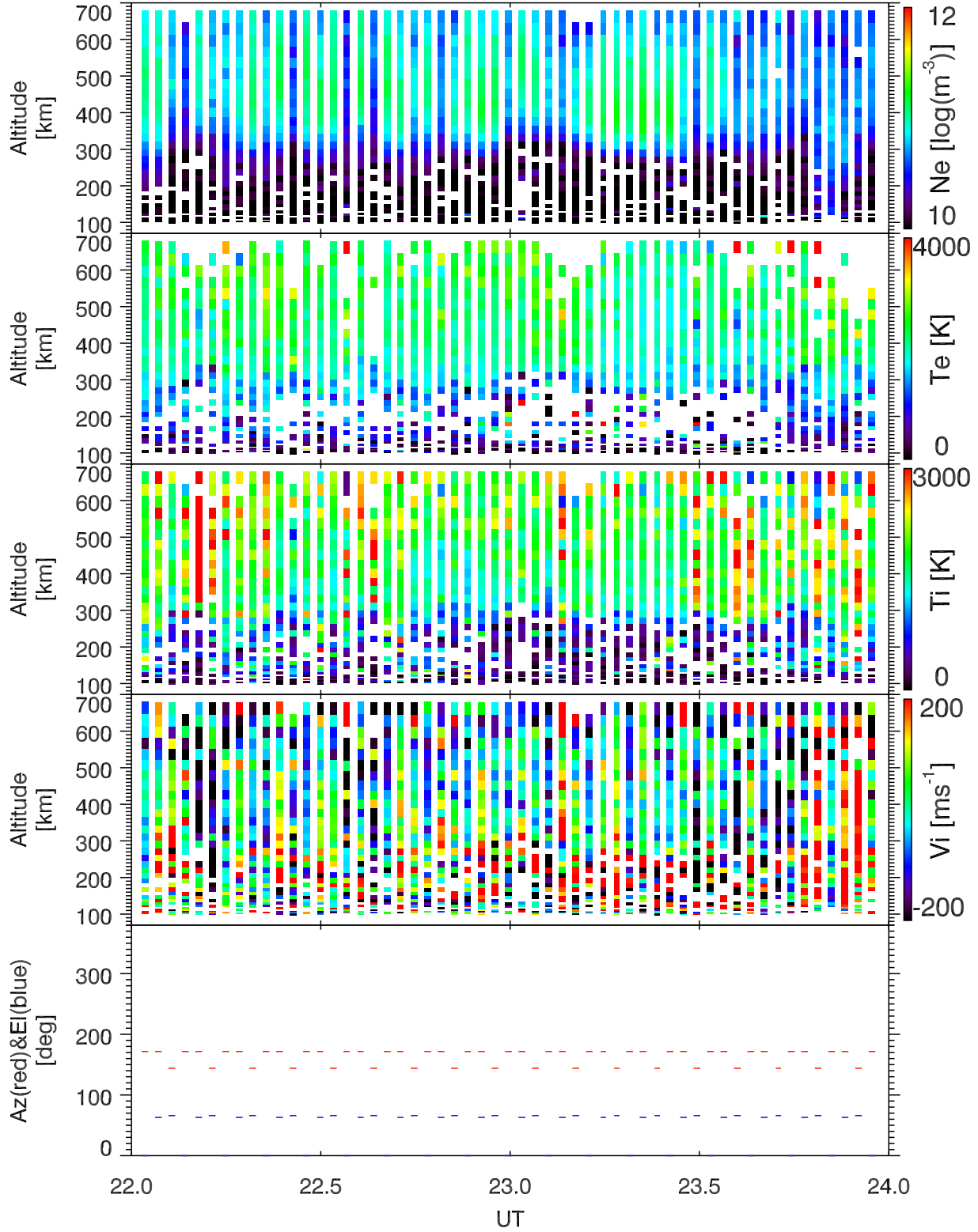
EISCAT 2002-10-15_22_24UT_tau0_ant@32m.
