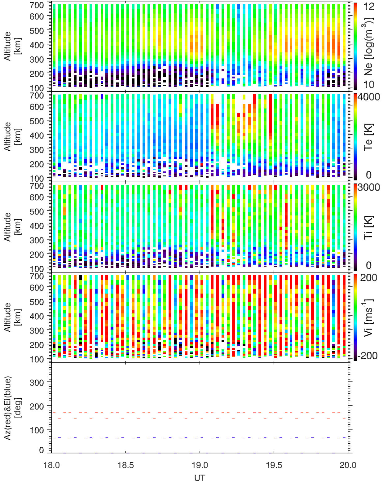
EISCAT 2002-10-16_18_20UT_tau0_ant@32m.
