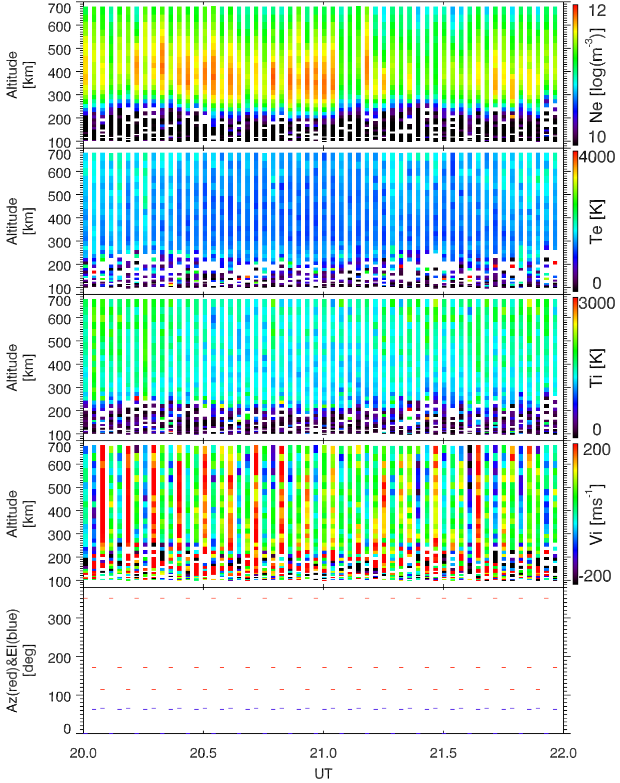
EISCAT 2002-10-17_20_22UT_tau0_ant@32m.
