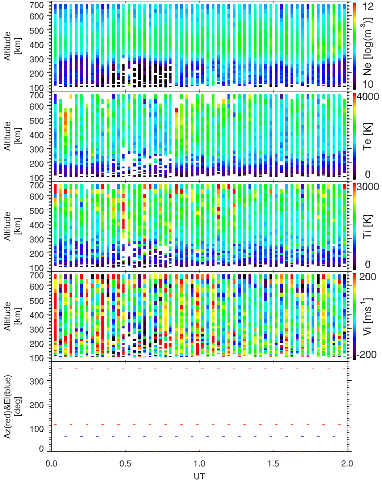
EISCAT 2002-10-18_00_02UT_tau0_ant@32m.
