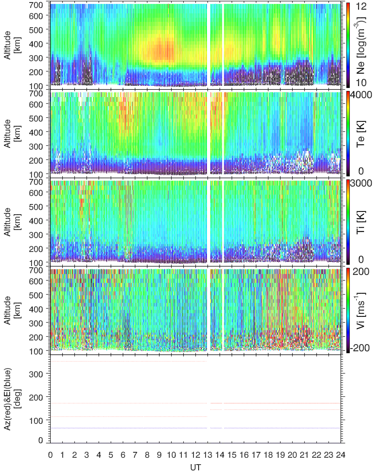
EISCAT 2002-10-18_00_24UT_tau0_ant@32m.
