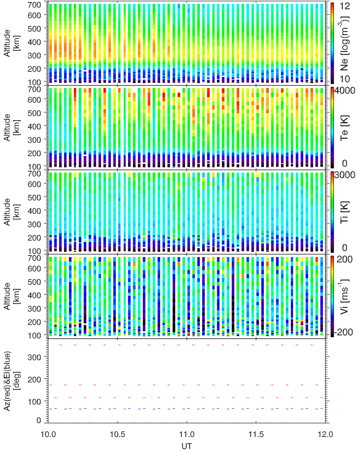
EISCAT 2002-10-18_10_12UT_tau0_ant@32m.
