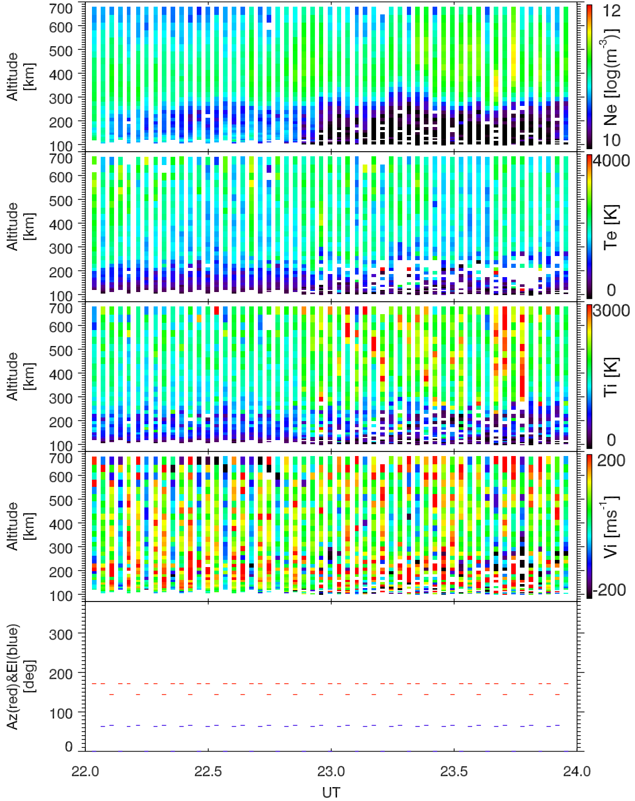
EISCAT 2002-10-18_22_24UT_tau0_ant@32m.
