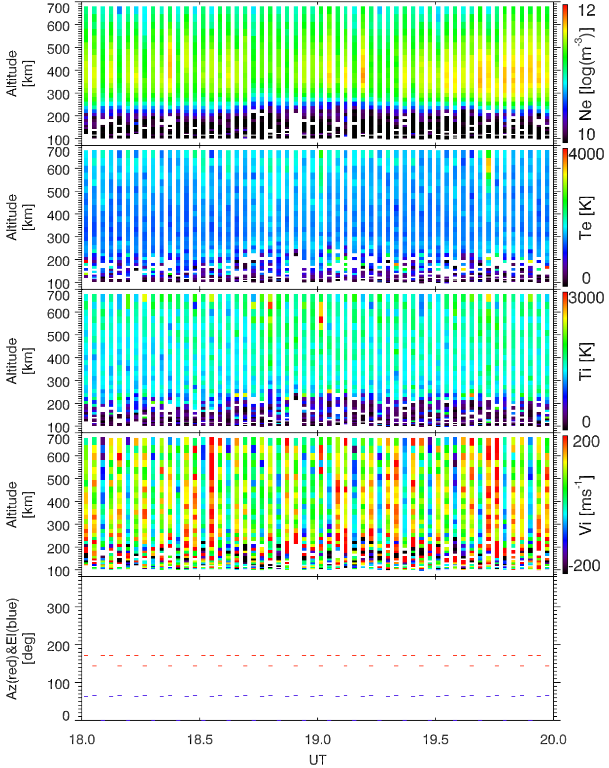
EISCAT 2002-10-19_18_20UT_tau0_ant@32m.
