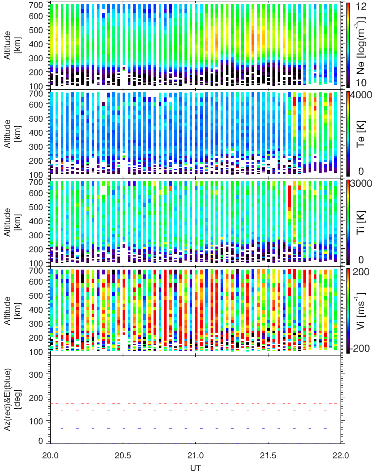
EISCAT 2002-10-19_20_22UT_tau0_ant@32m.
