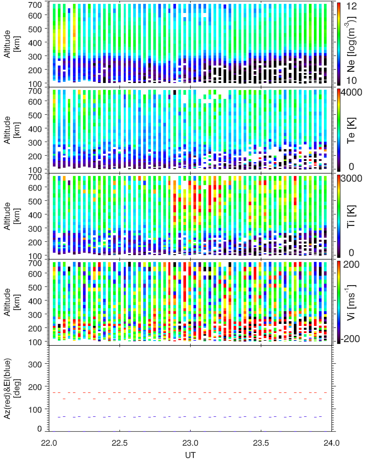
EISCAT 2002-10-19_22_24UT_tau0_ant@32m.
