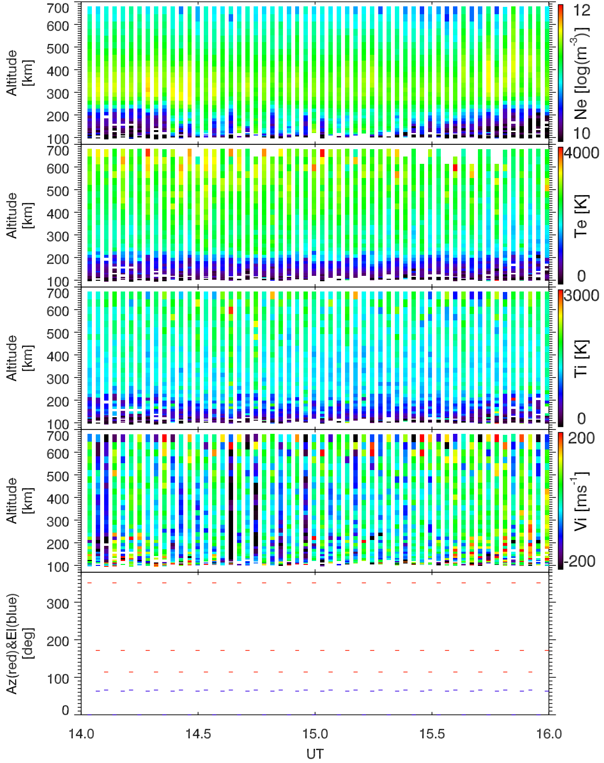
EISCAT 2002-10-20_14_16UT_tau0_ant@32m.
