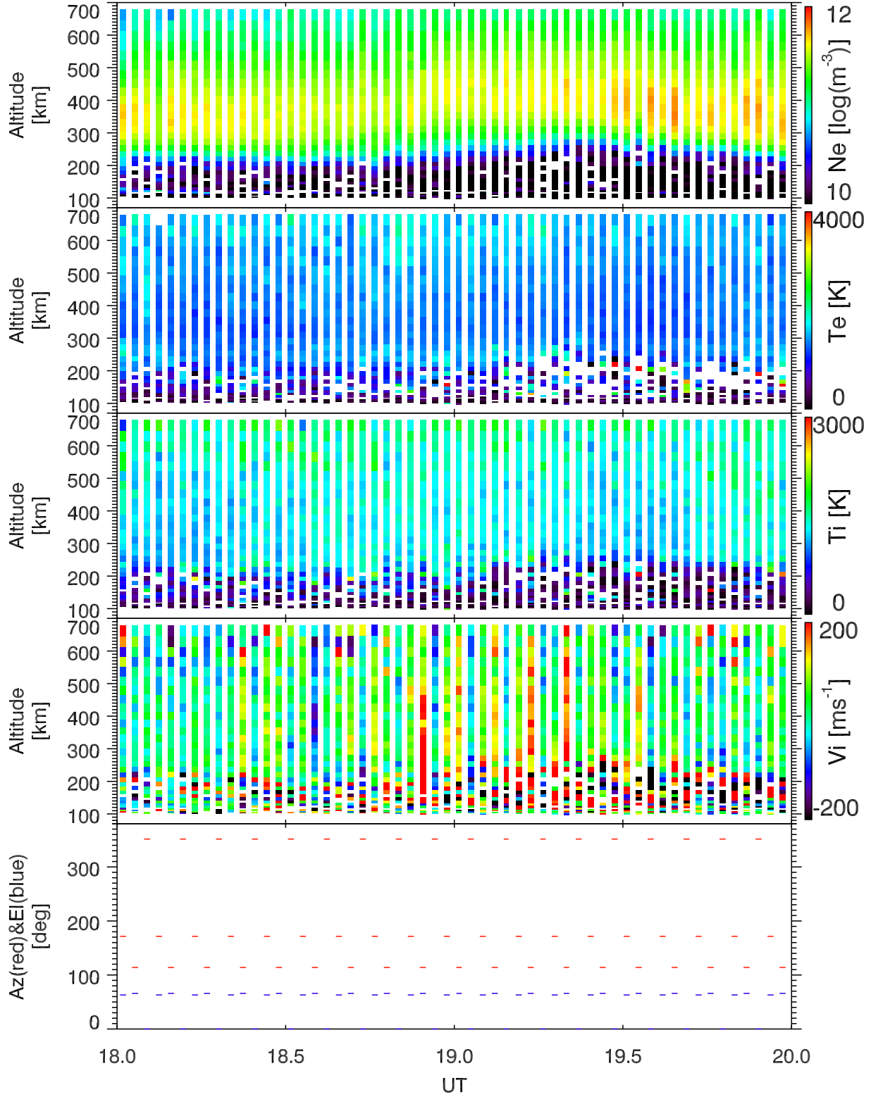
EISCAT 2002-10-20_18_20UT_tau0_ant@32m.
