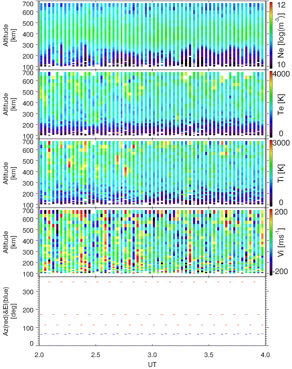
EISCAT 2002-10-21_02_04UT_tau0_ant@32m.
