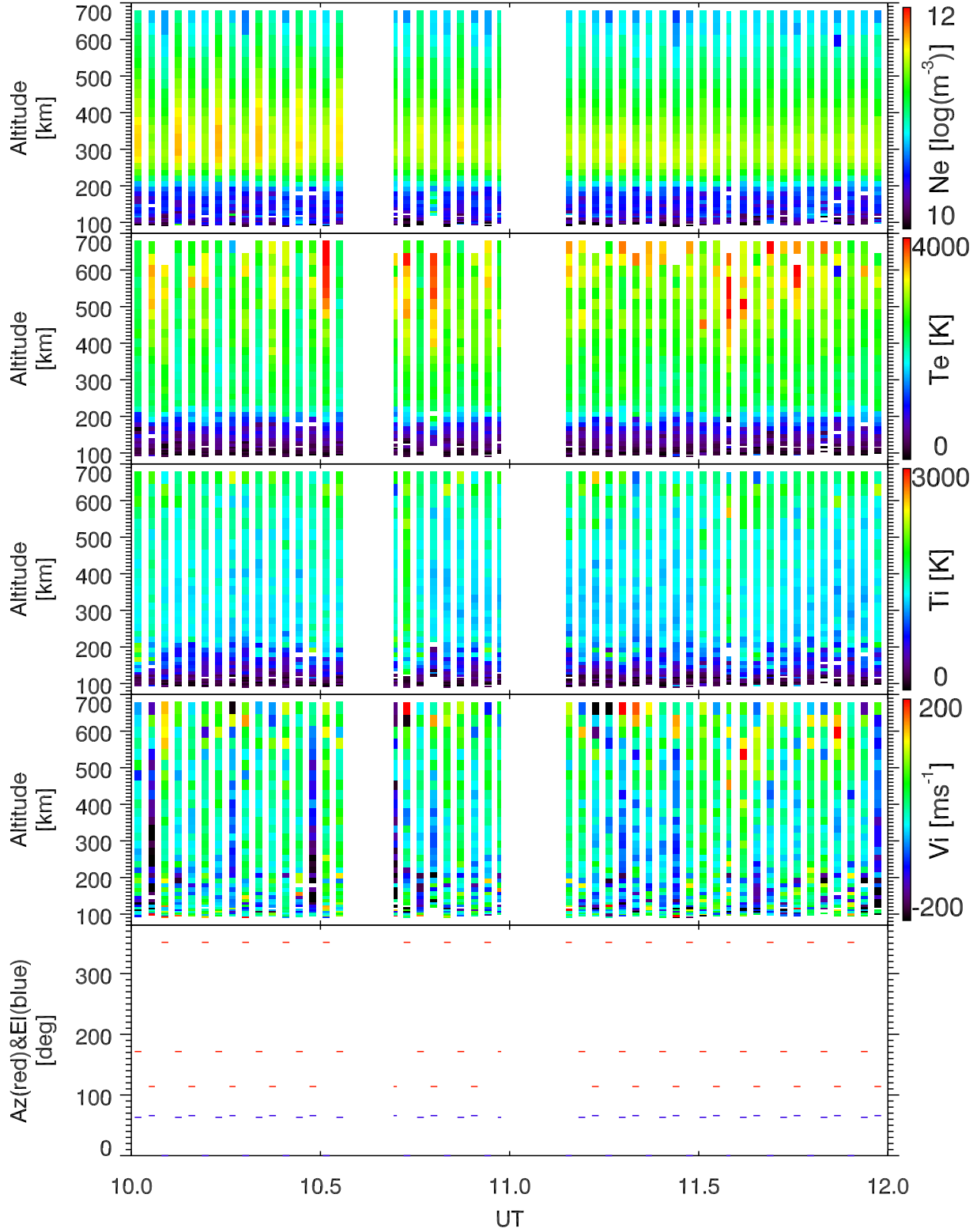
EISCAT 2002-10-21_10_12UT_tau0_ant@32m.
