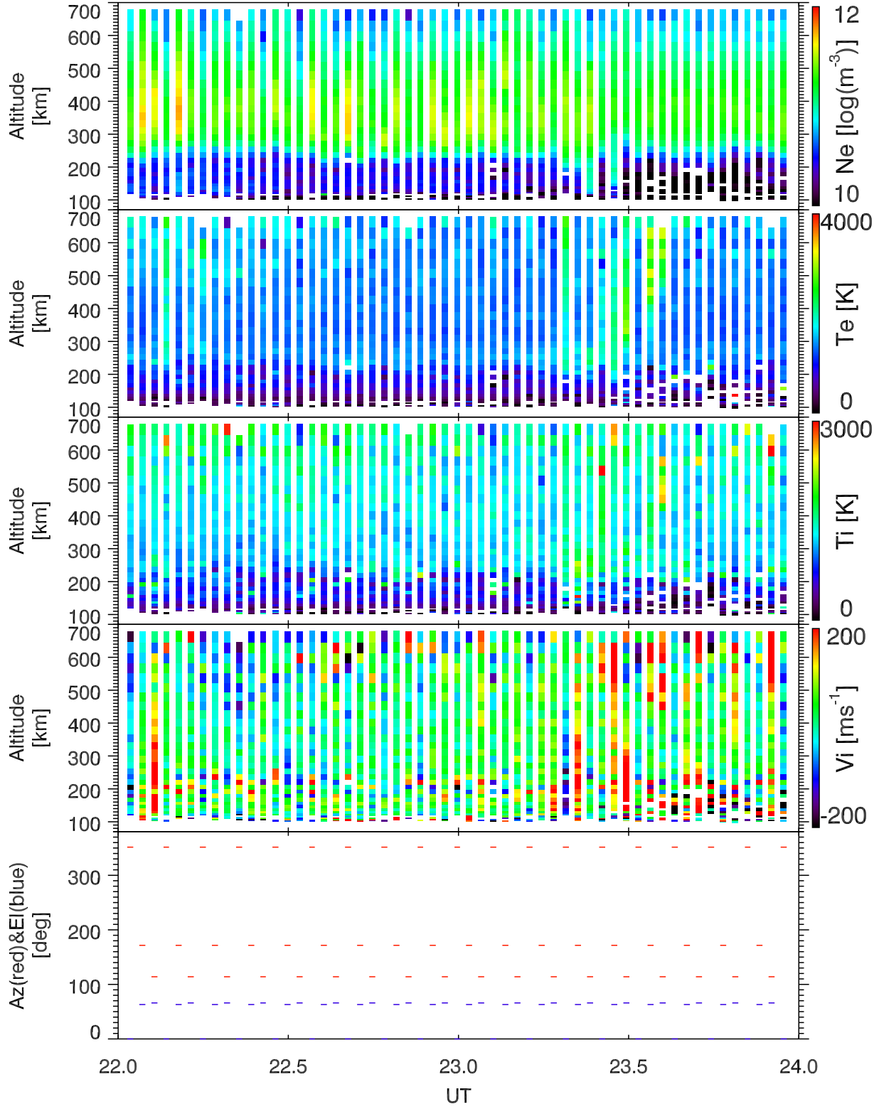
EISCAT 2002-10-21_22_24UT_tau0_ant@32m.
