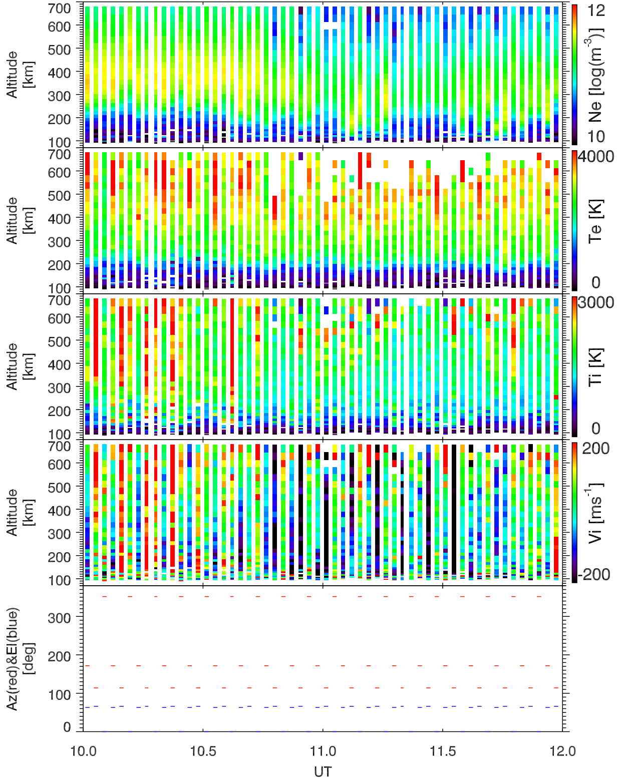
EISCAT 2002-10-22_10_12UT_tau0_ant@32m.
