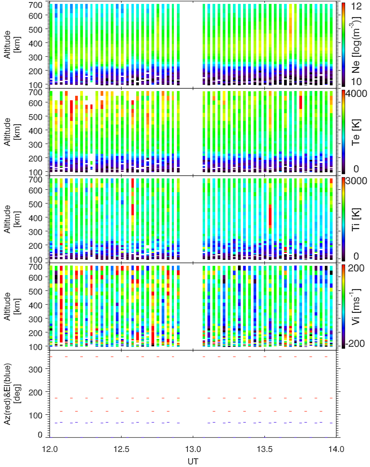
EISCAT 2002-10-22_12_14UT_tau0_ant@32m.
