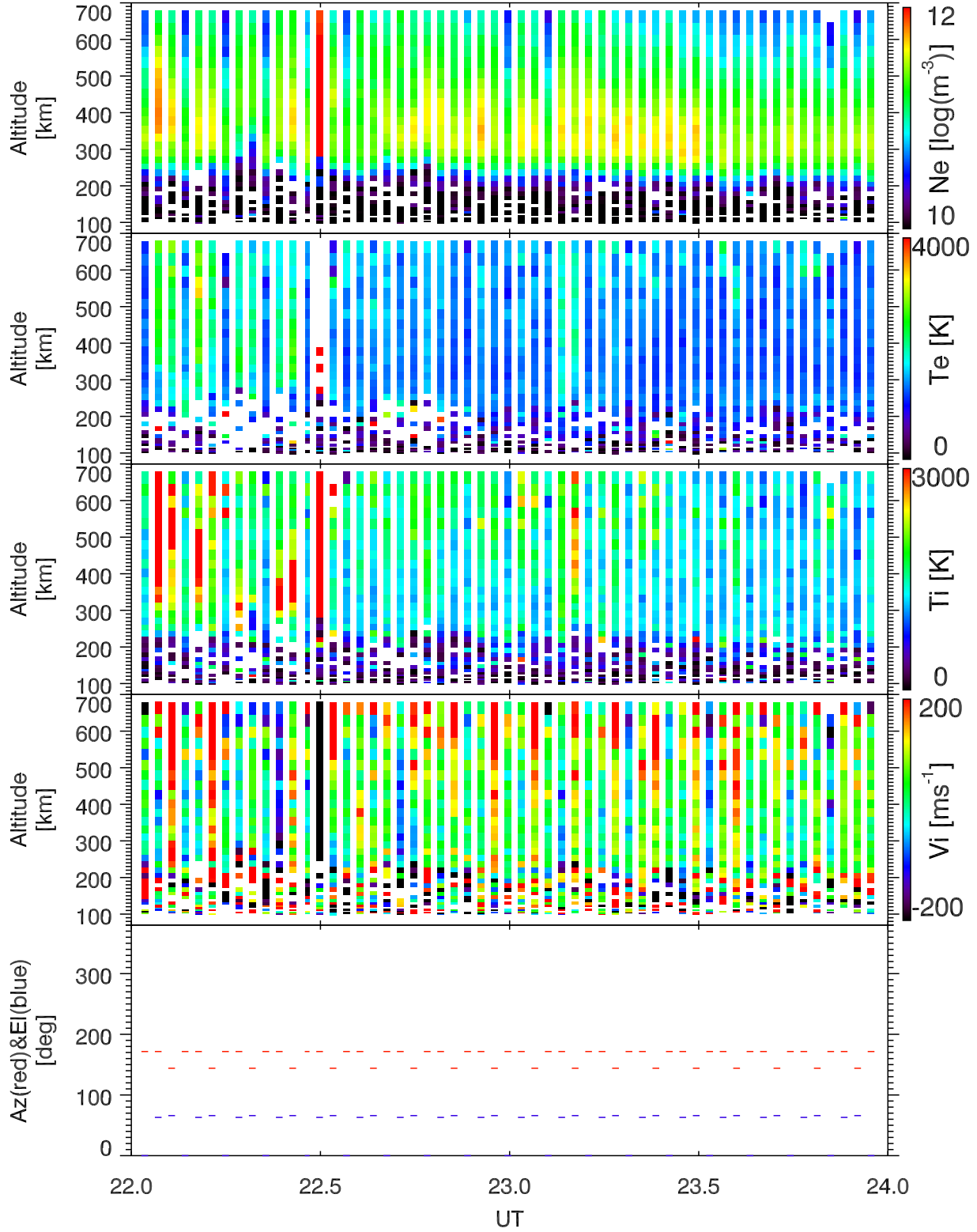
EISCAT 2002-10-22_22_24UT_tau0_ant@32m.
