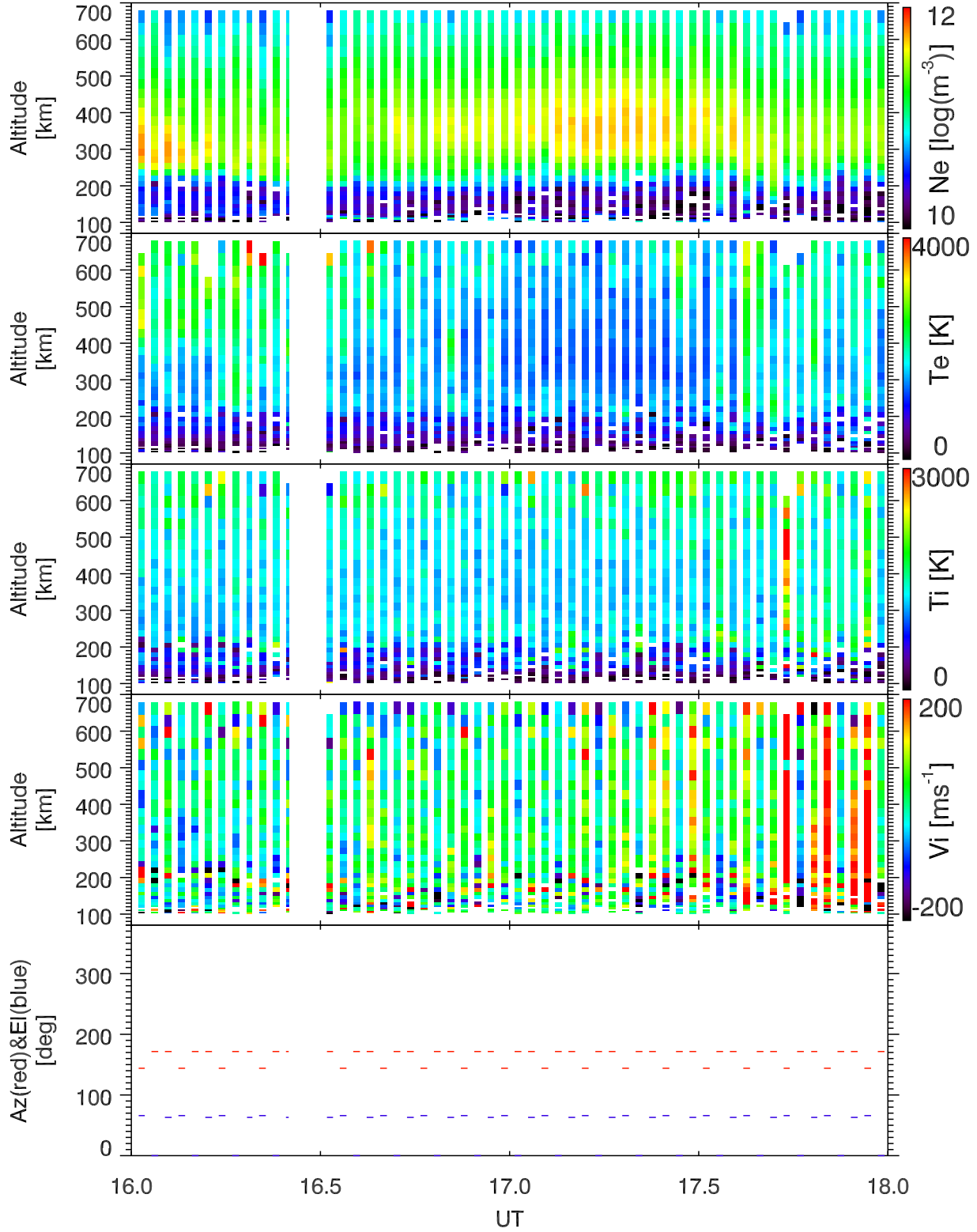
EISCAT 2002-10-23_16_18UT_tau0_ant@32m.
