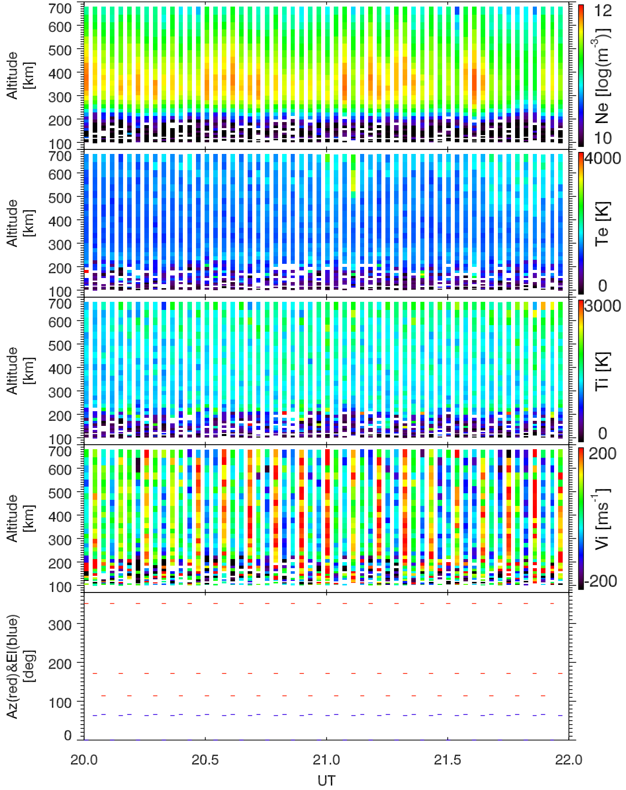
EISCAT 2002-10-23_20_22UT_tau0_ant@32m.
