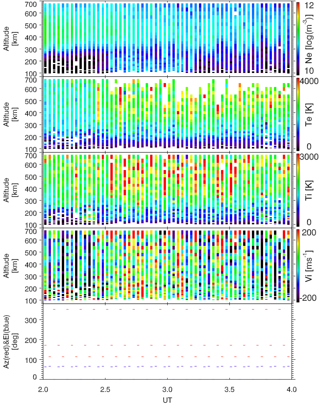
EISCAT 2002-10-24_02_04UT_tau0_ant@32m.
