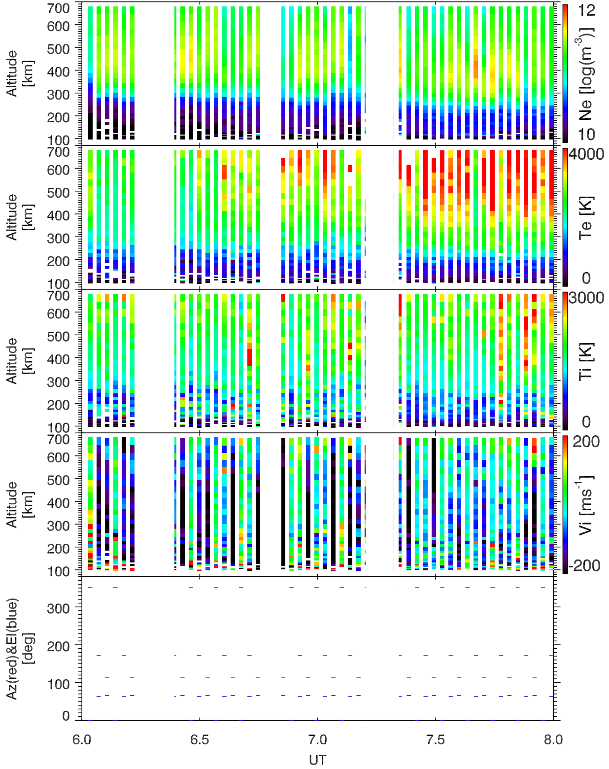
EISCAT 2002-10-24_06_08UT_tau0_ant@32m.
