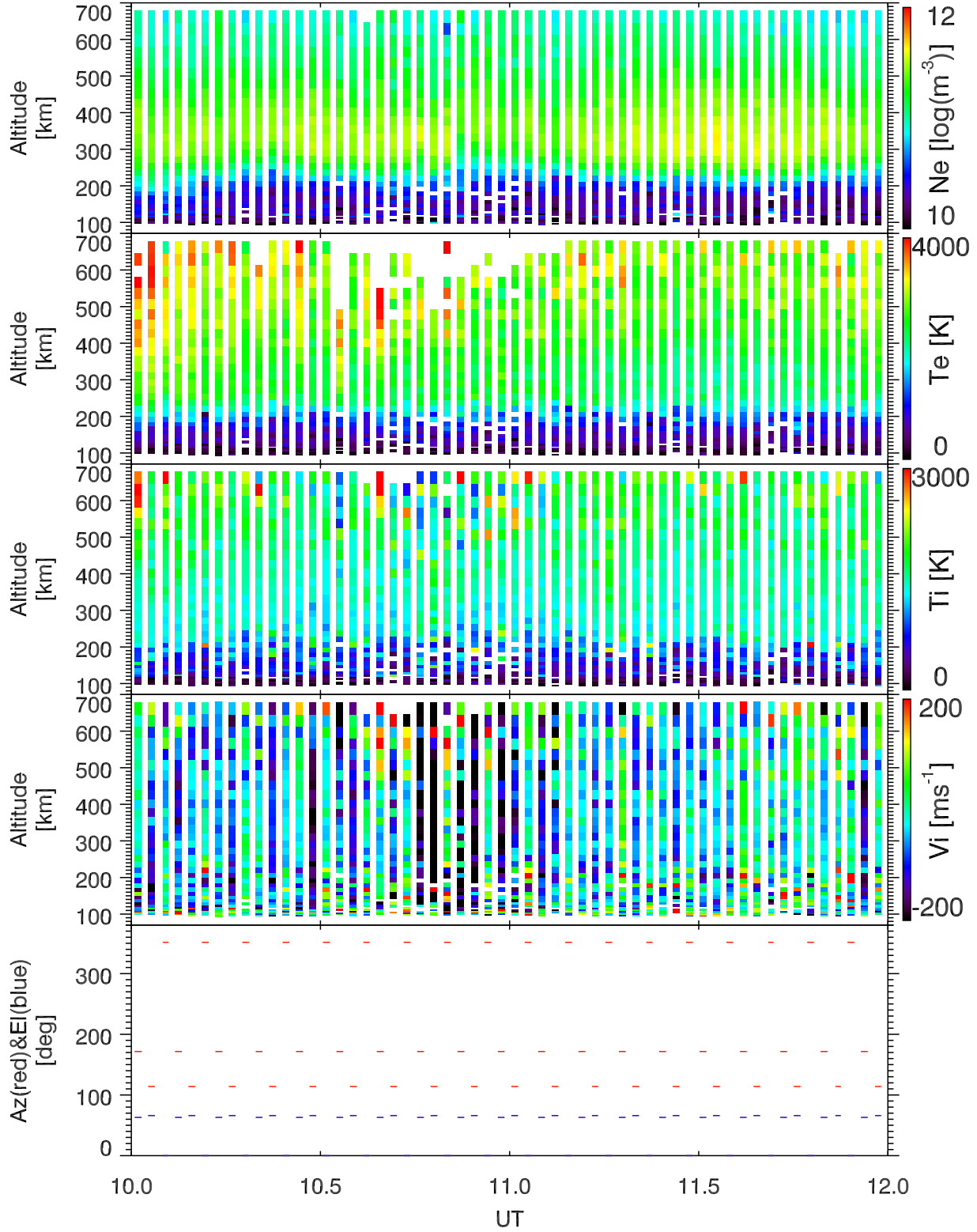
EISCAT 2002-10-24_10_12UT_tau0_ant@32m.
