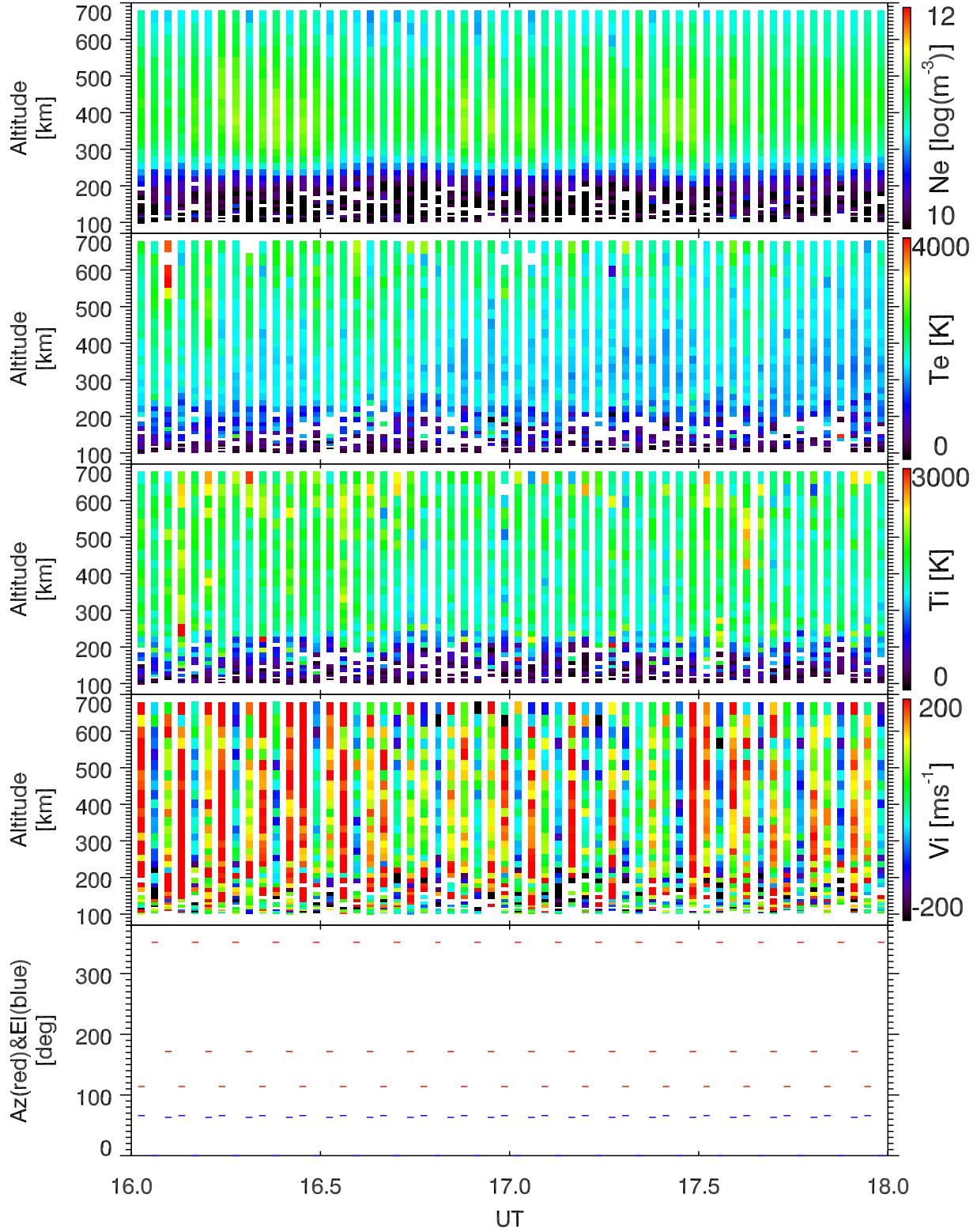
EISCAT 2002-10-24_16_18UT_tau0_ant@32m.
