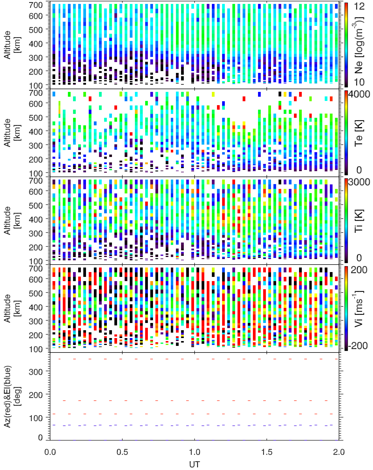
EISCAT 2002-10-25_00_02UT_tau0_ant@32m.
