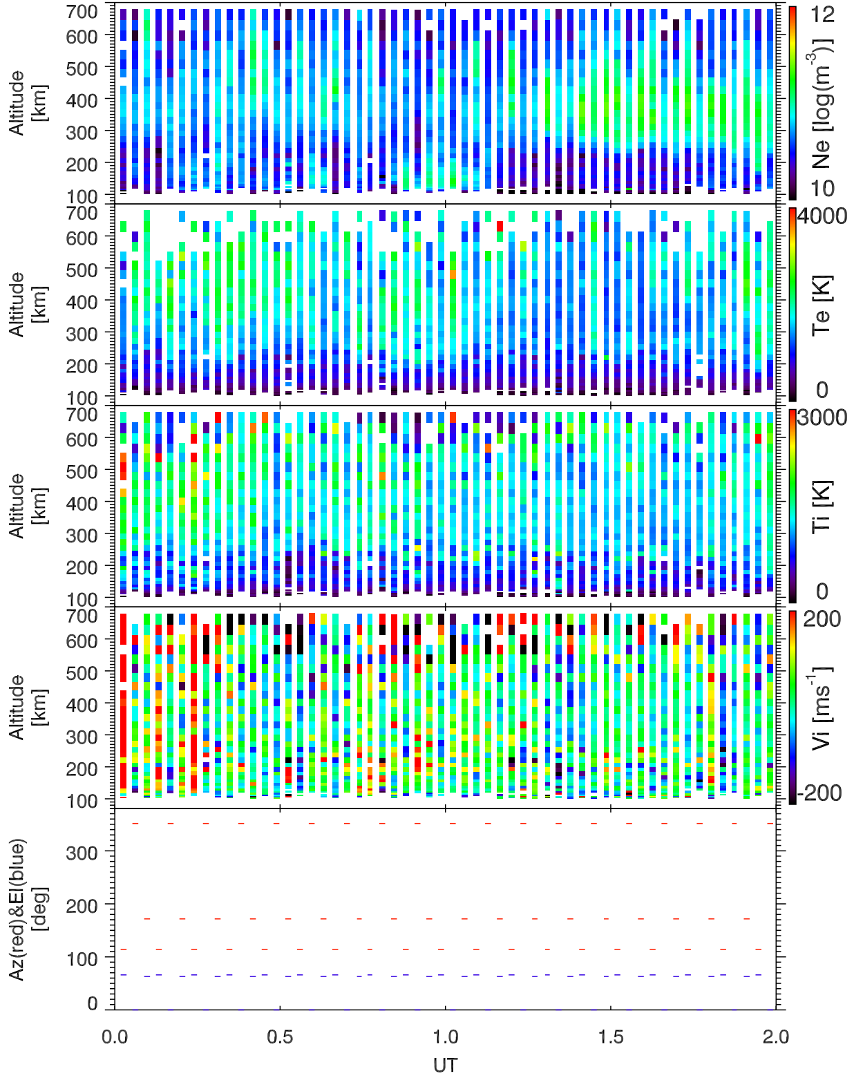
EISCAT 2002-10-26_00_02UT_tau0_ant@32m.
