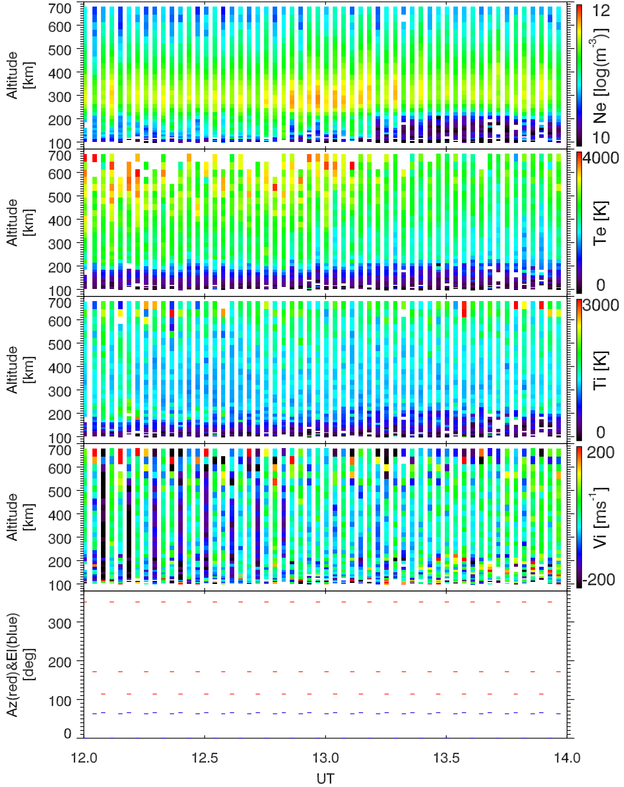
EISCAT 2002-10-26_12_14UT_tau0_ant@32m.
