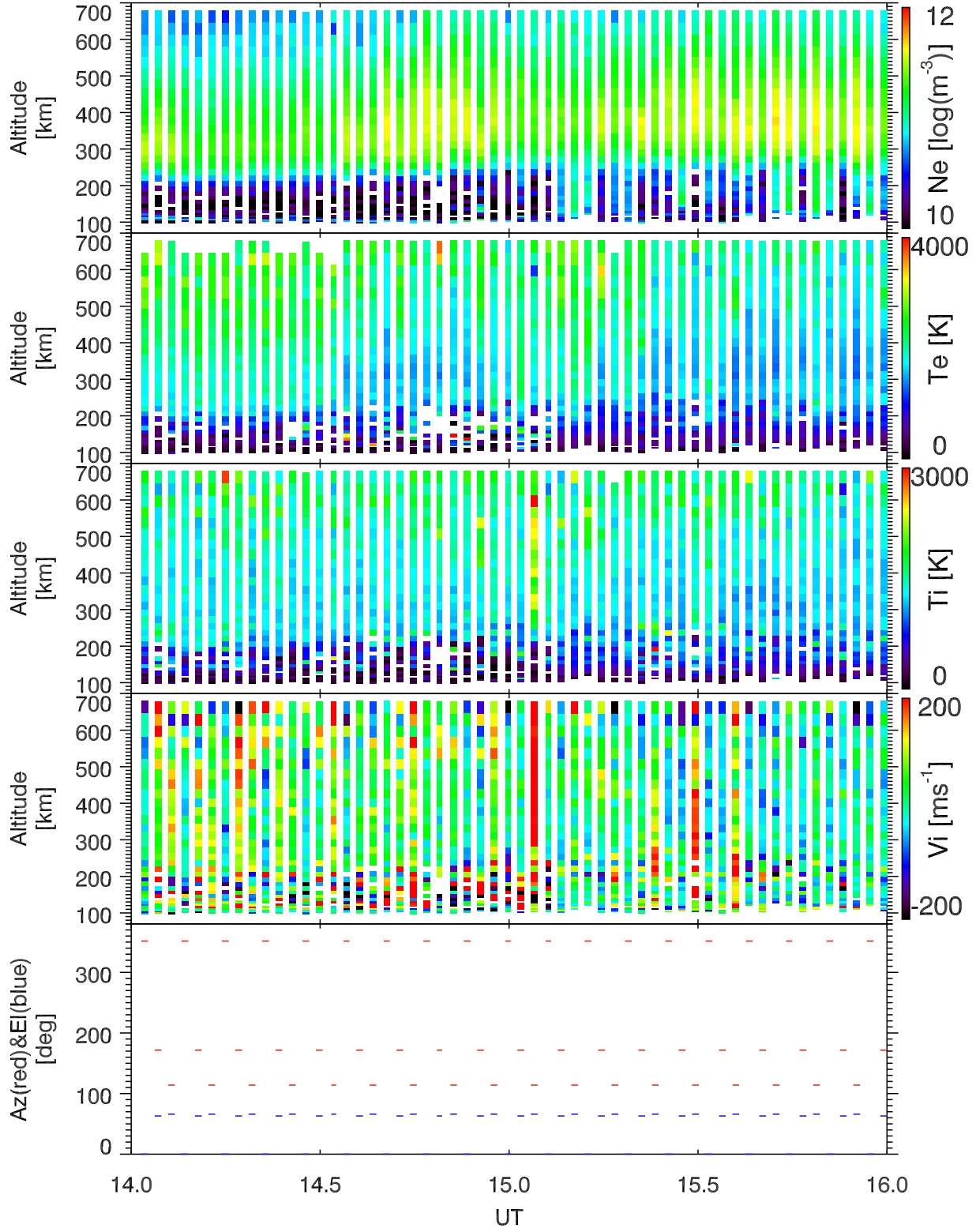
EISCAT 2002-10-26_14_16UT_tau0_ant@32m.
