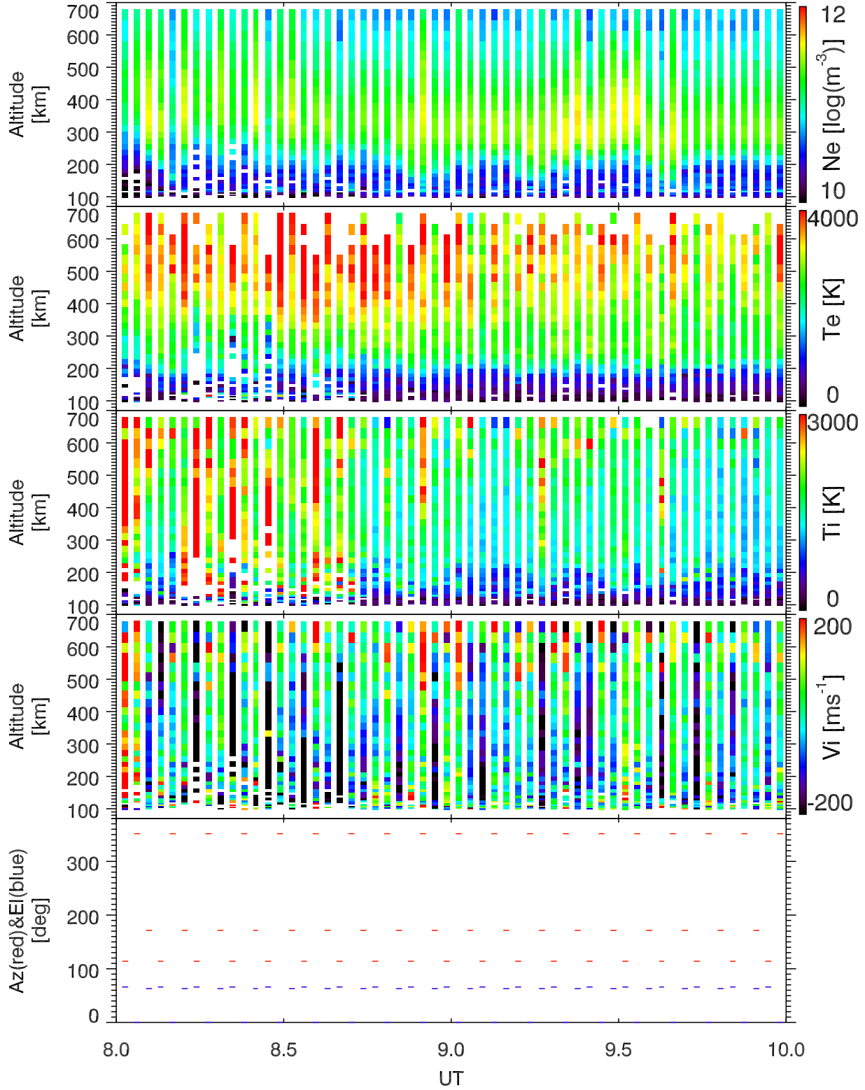
EISCAT 2002-10-27_08_10UT_tau0_ant@32m.
