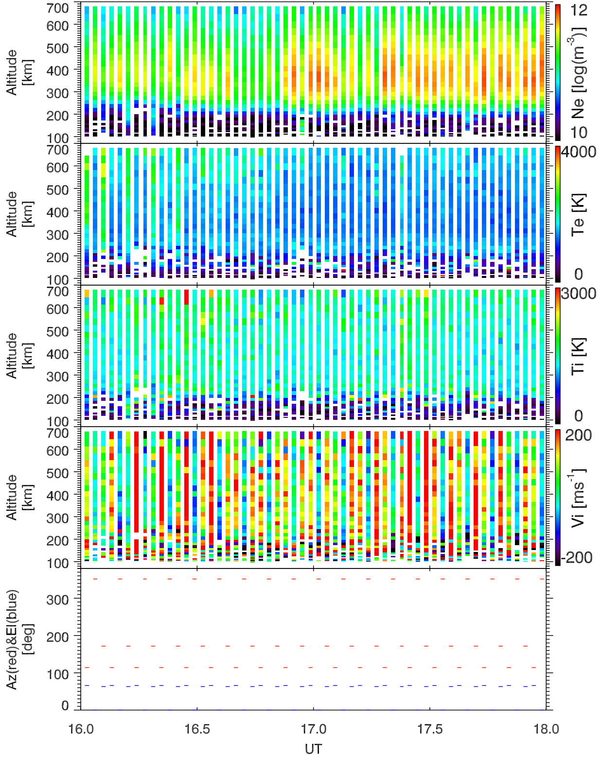
EISCAT 2002-10-27_16_18UT_tau0_ant@32m.
