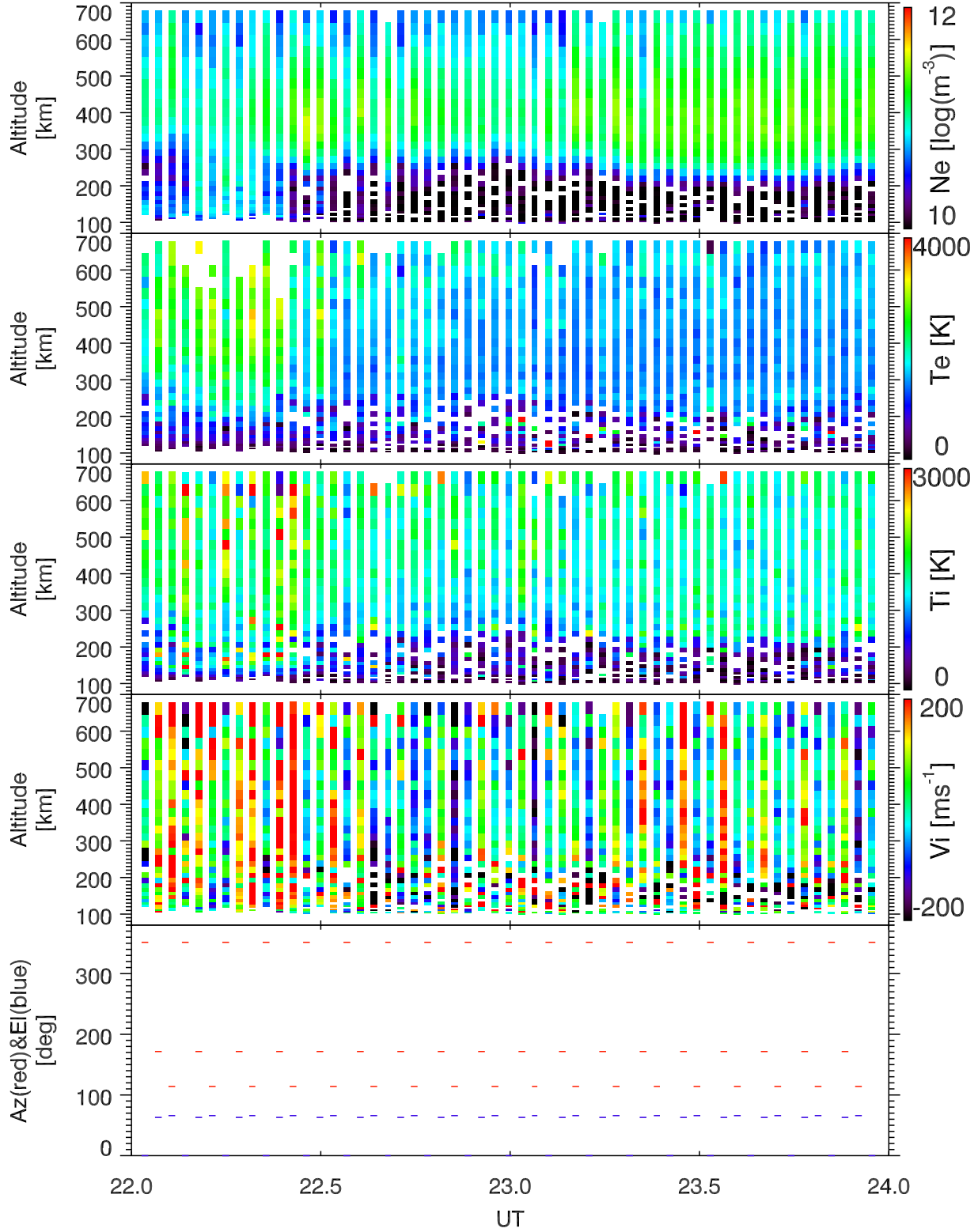
EISCAT 2002-10-27_22_24UT_tau0_ant@32m.
