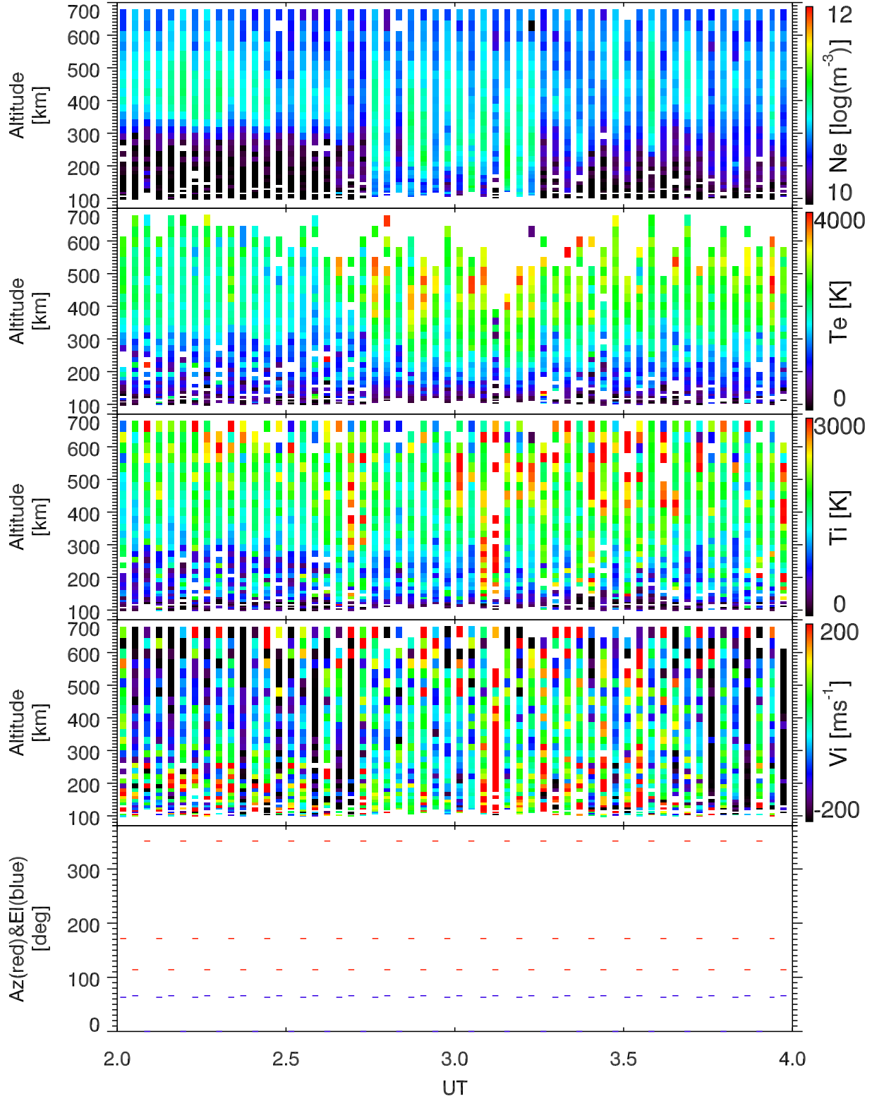
EISCAT 2002-10-28_02_04UT_tau0_ant@32m.
