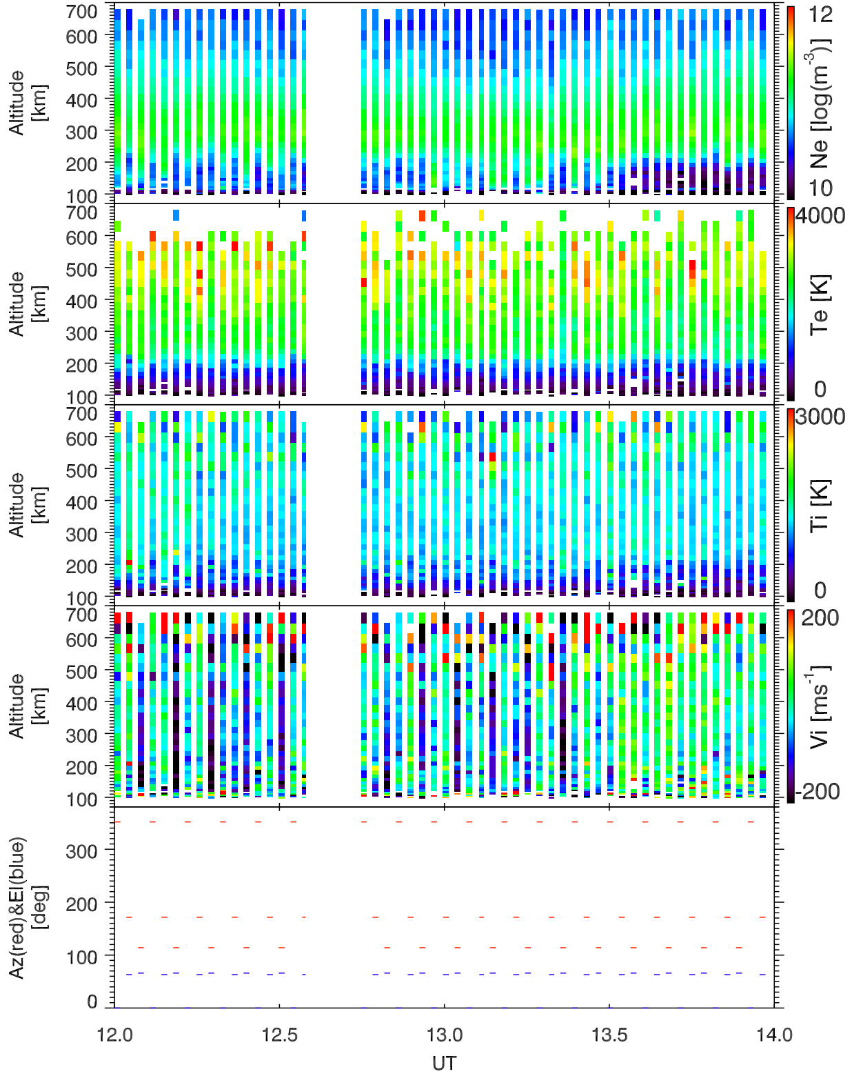
EISCAT 2002-10-29_12_14UT_tau0_ant@32m.
