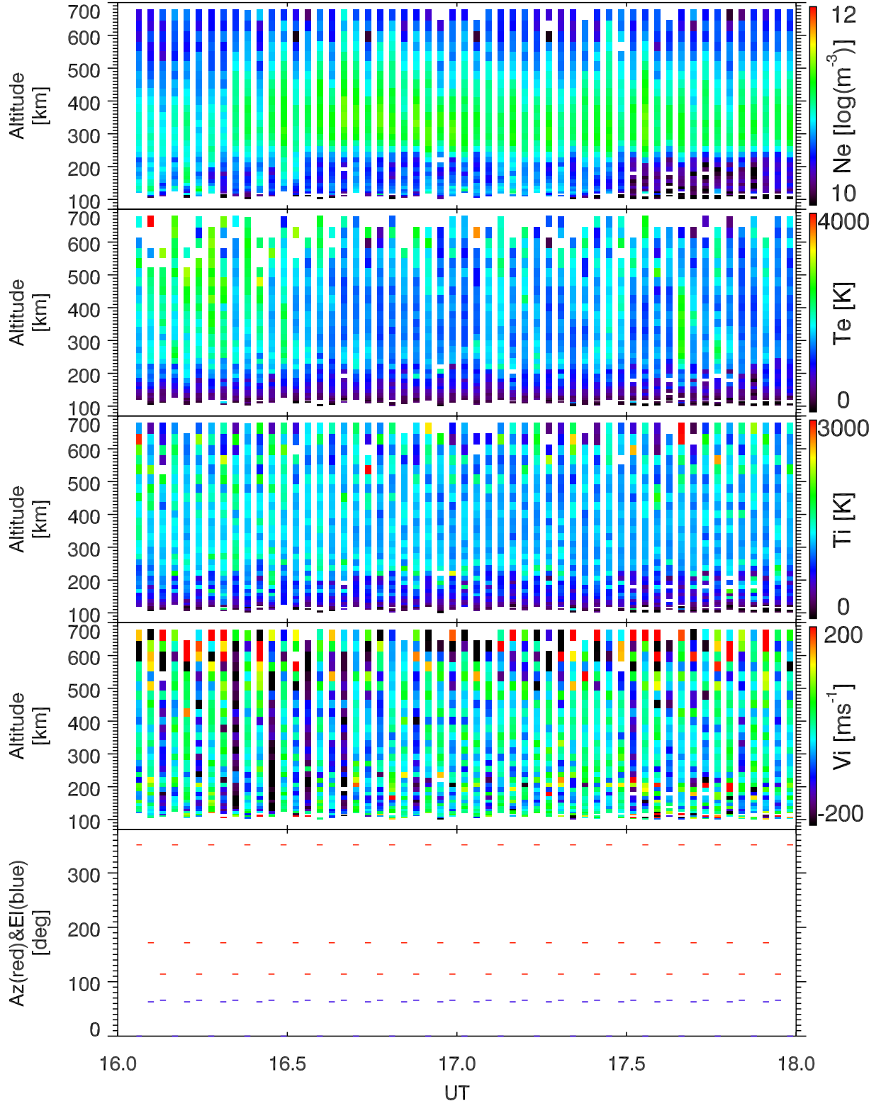
EISCAT 2002-10-29_16_18UT_tau0_ant@32m.
