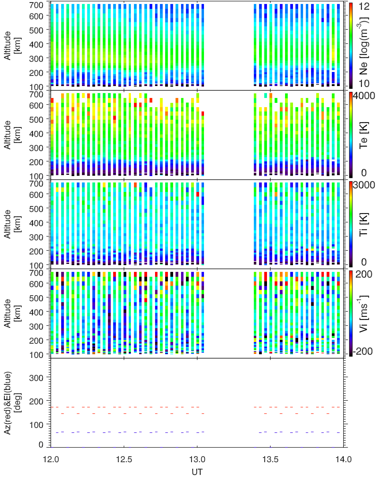
EISCAT 2002-10-30_12_14UT_tau0_ant@32m.
