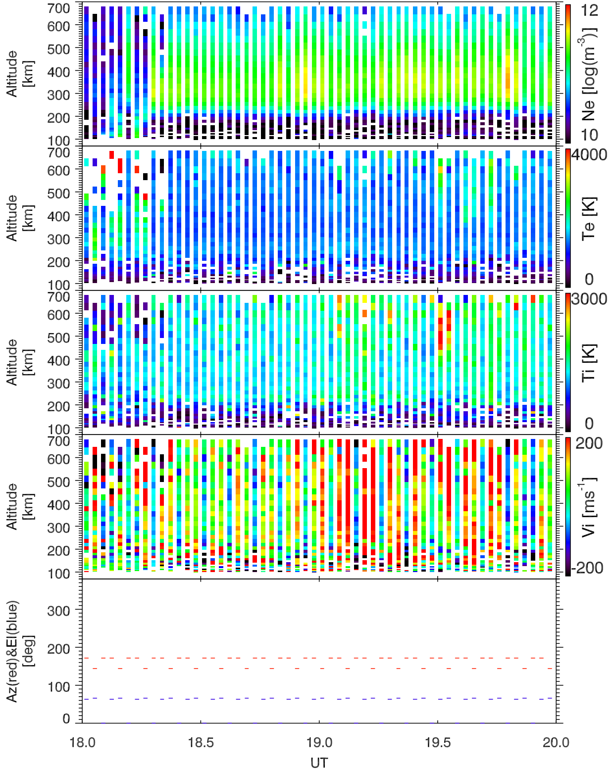
EISCAT 2002-10-30_18_20UT_tau0_ant@32m.
