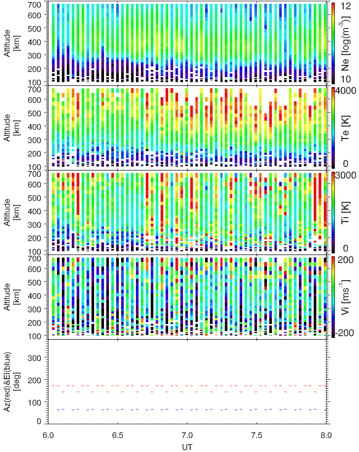
EISCAT 2002-10-31_06_08UT_tau0_ant@32m.
