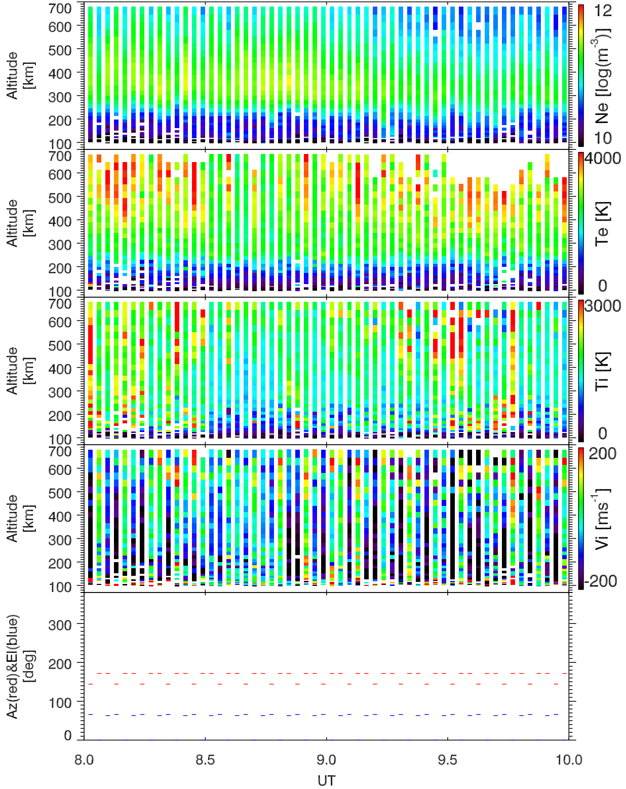
EISCAT 2002-10-31_08_10UT_tau0_ant@32m.
