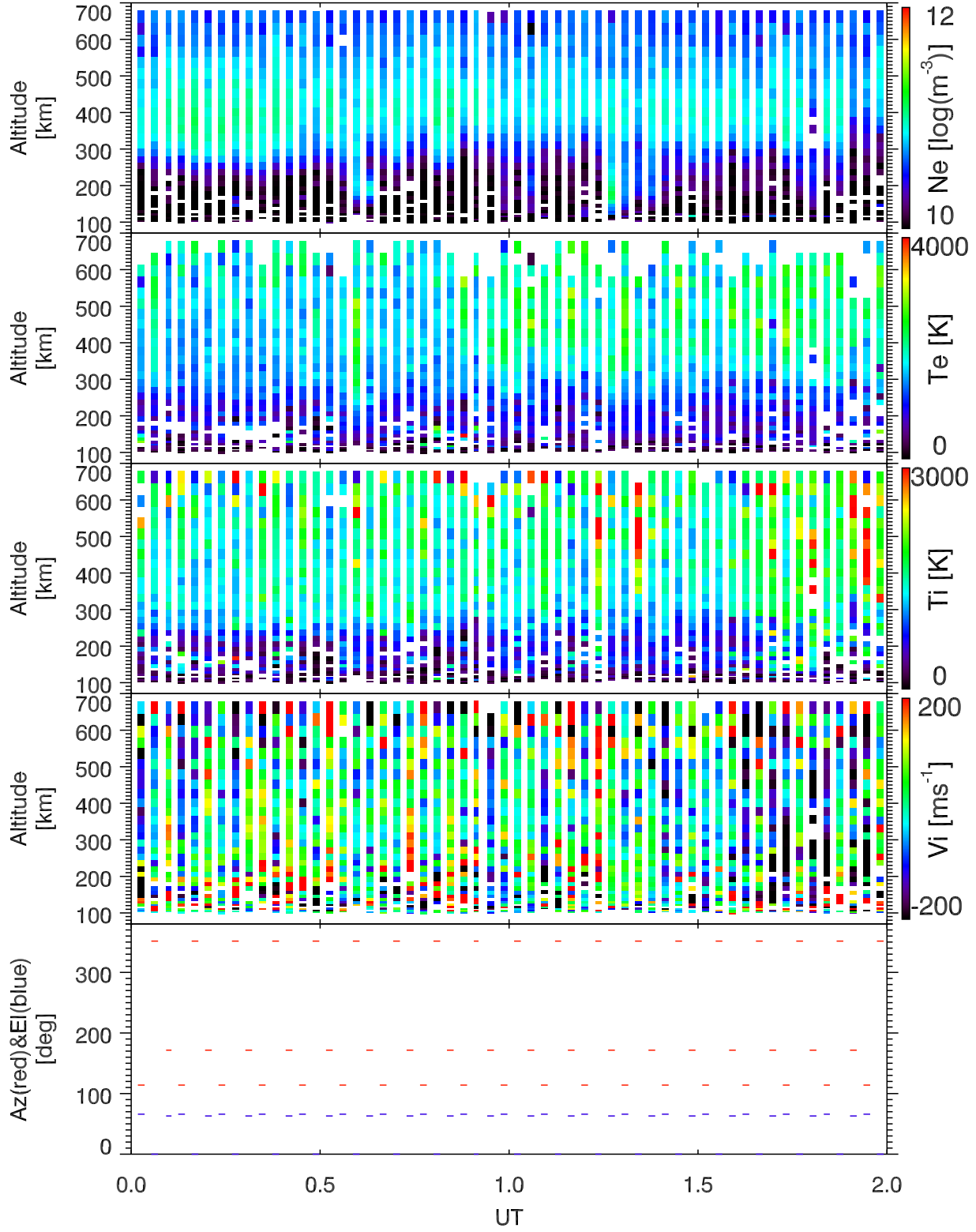
EISCAT 2002-11-01_00_02UT_tau0_ant@32m.
