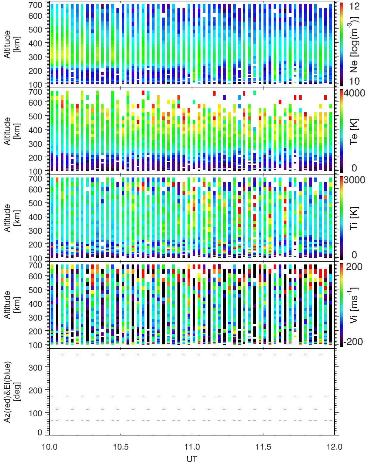
EISCAT 2002-11-01_10_12UT_tau0_ant@32m.
